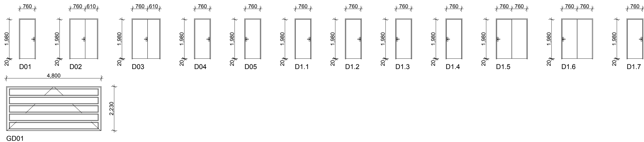
Internal Joinery and Garage Door Schedule 1:100
