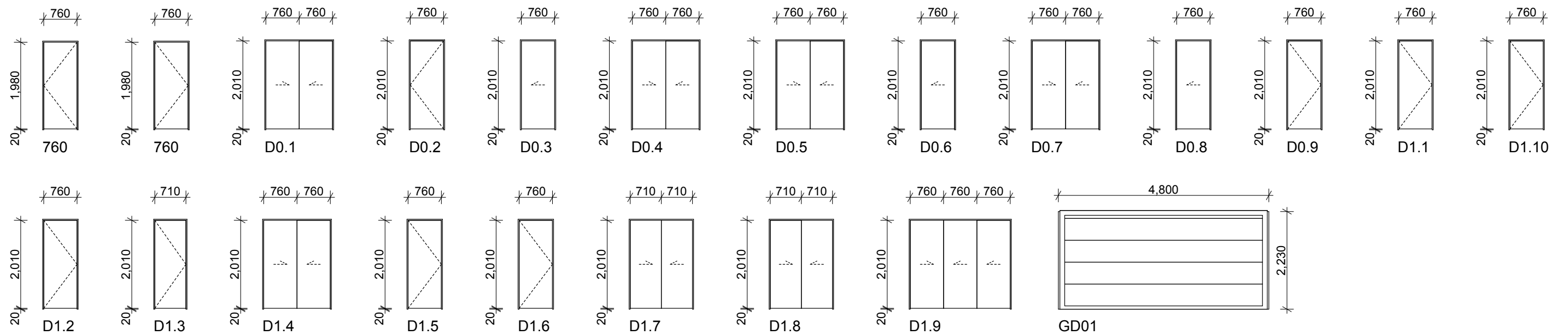
Internal Joinery and Garage Door Schedule 1:100
