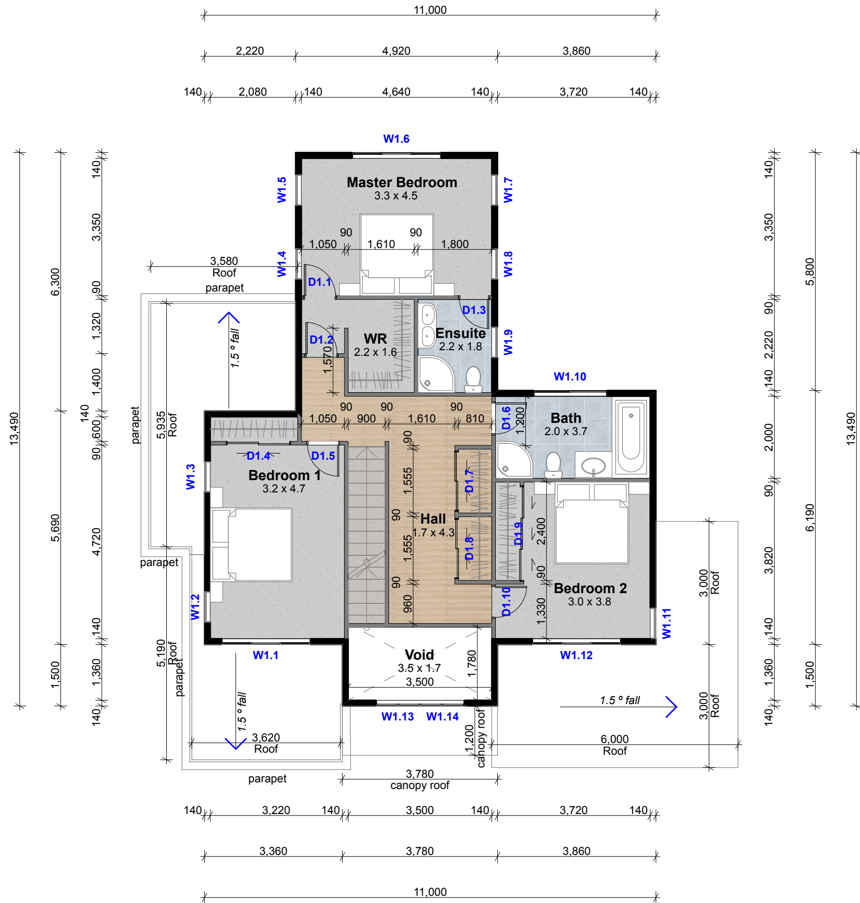
First Floor Plan Wall Set-out 1:100
