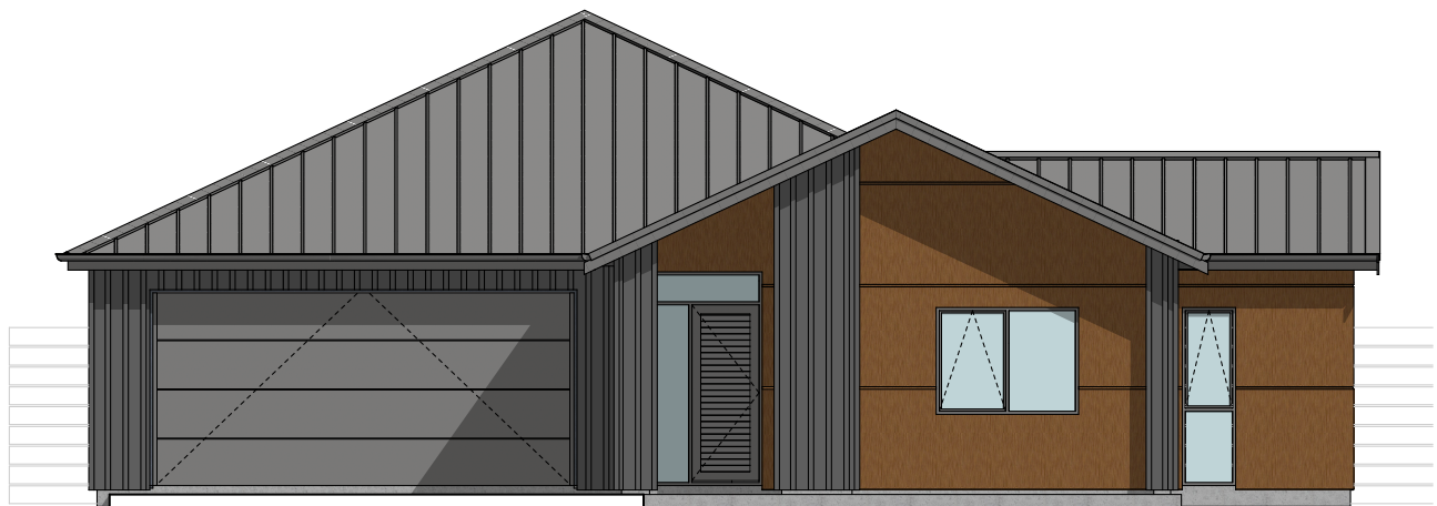
F Front Elevation 1:100
