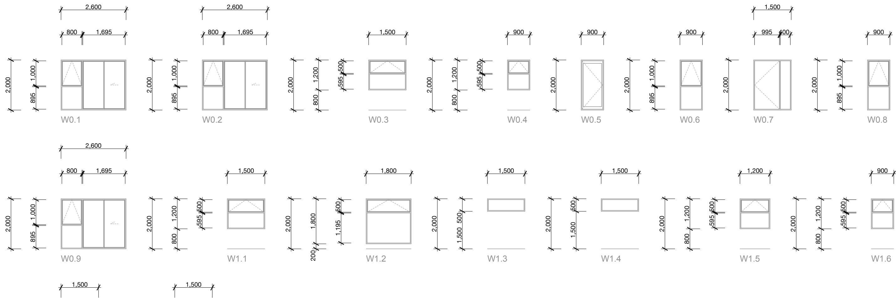
External Joinery Schedule 1:100
