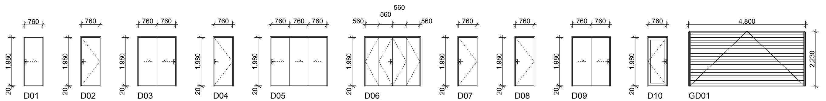
Internal Joinery and Garage Door Schedule 1:100
