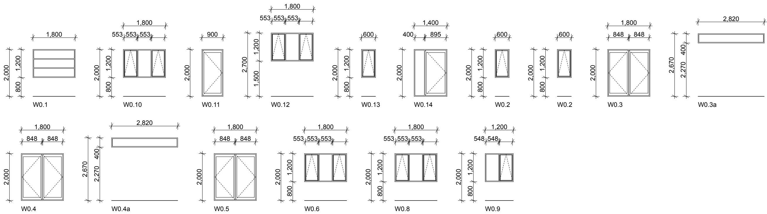
External Joinery Schedule 1:100
