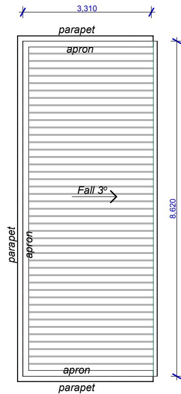
Roof Plan 1:100
